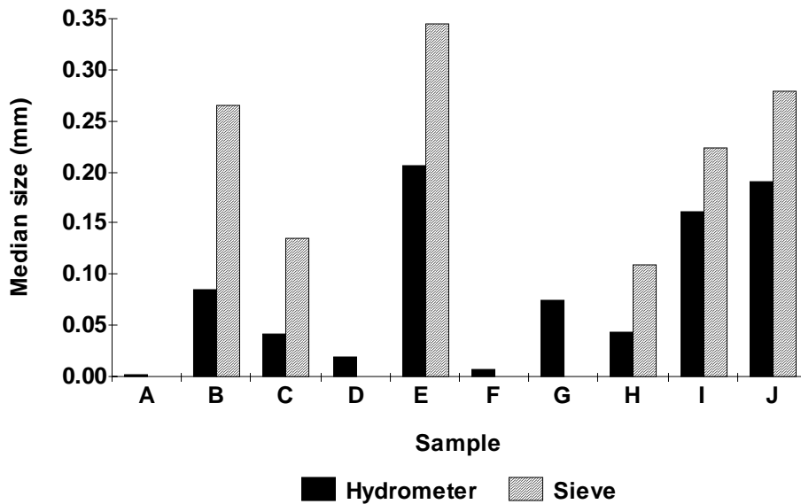
Figure 8. Comparison of the median size (d50) of river and flood plain sediment from the Rio Puerco as determined from hydrometer analysis using a dispersant and from dry sieving.
