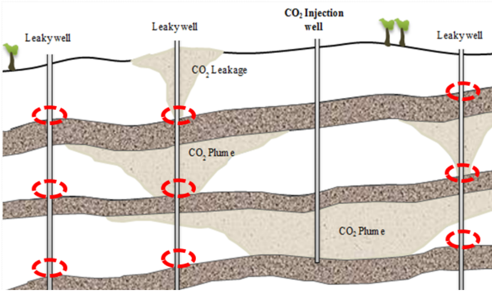
Figure 2. Pressure unknowns for this domain are located at the red circles
